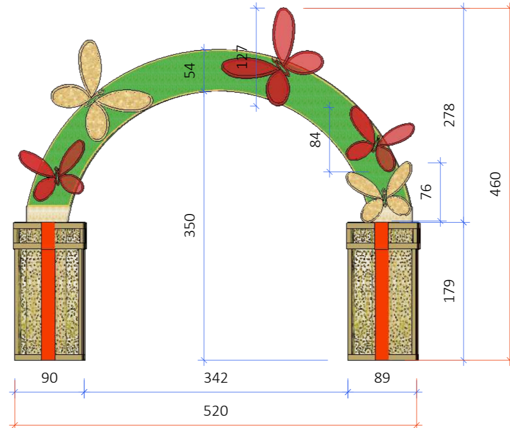
VISTA FRONTAL
